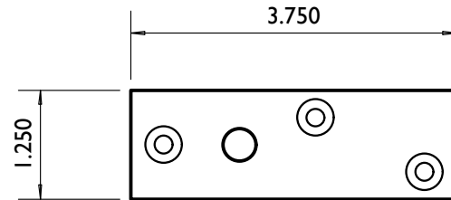
PLAN VIEW: DOOR PLATE # CF-410-3
